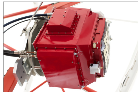
FIGURE 2: GCT CAMERA
